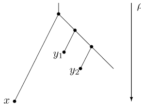
Fig. 14. A situation in which necessarily d(x, y_1) = d(x, y_2) .
