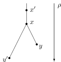
Fig. 13. Monotonicity and Submodularity of d .
