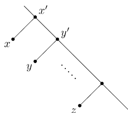
Fig. 3. A restriction of the cladistic model.
