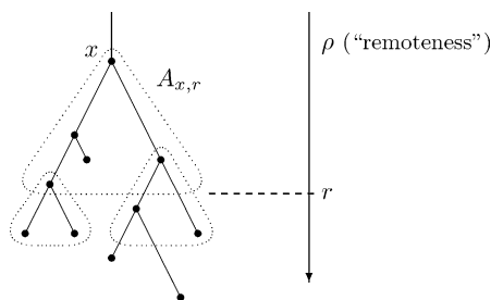
Fig. 11. Graphic Representation of \mathcal{PH}_\rho .
