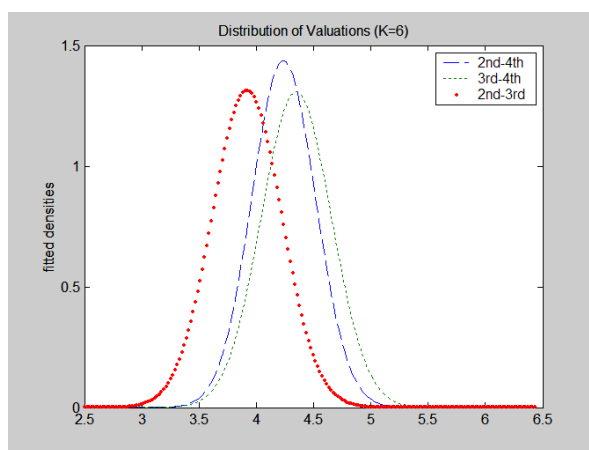
FIGURE 2: Estimated density function with K = 6 for the wholesale used-car auction data
