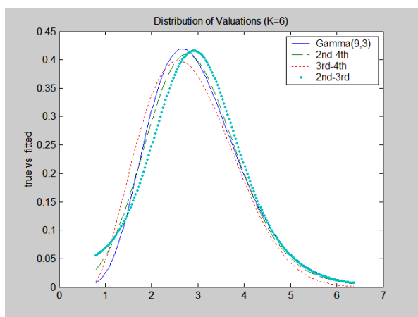
FIGURE 1: Estimated density function with K = 6 for a Monte Carlo simulated data
